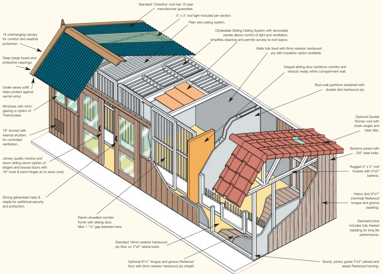
ILLUSTRATION SHOWS STANDARD CLYDESDALE 3-SECTION CORRIDOR LOFT WITH AVAILABLE OPTIONS. (BASE NOT SUPPLIED)
